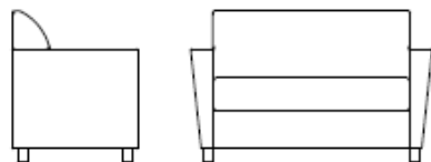
SF8302 University Loveseat, Closed Front Front 27"d x 52"w x 33.5"h 24.5" arm ht 19" seat ht
